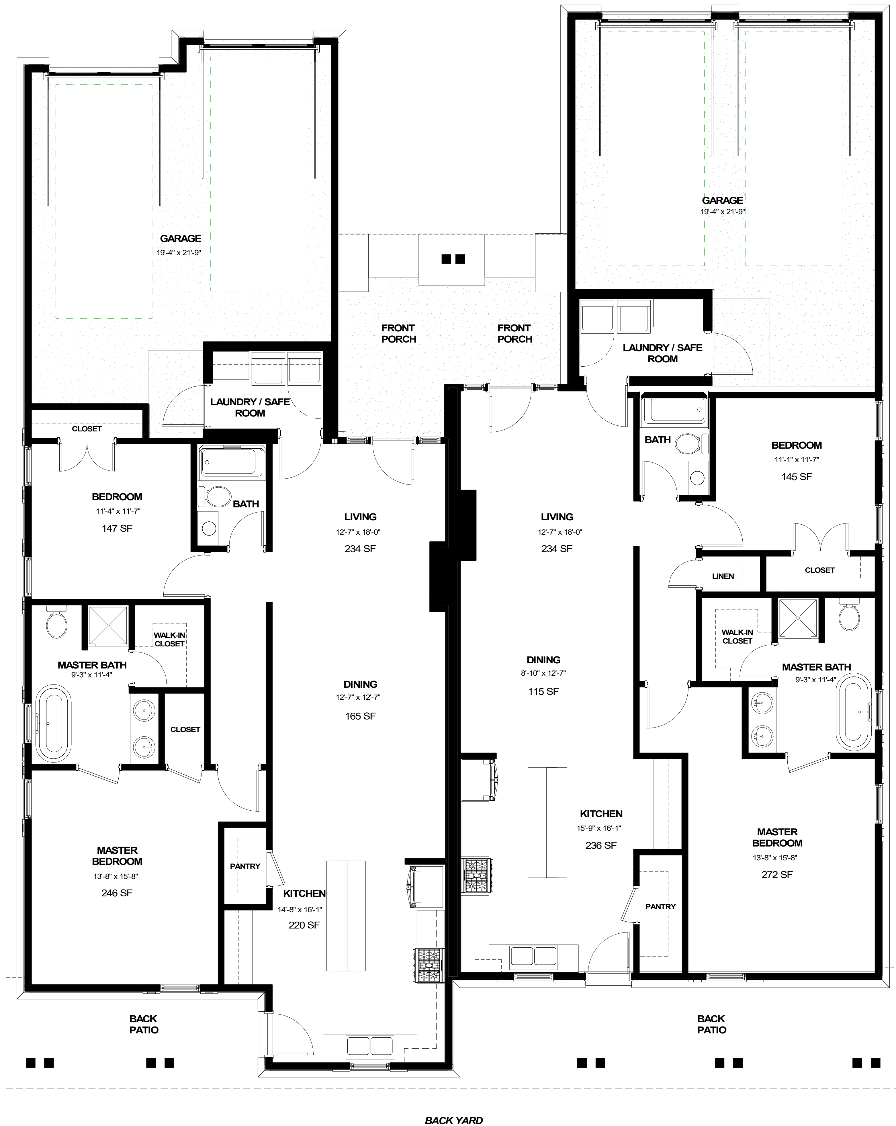
VILLA 'A' FLOOR PLAN
