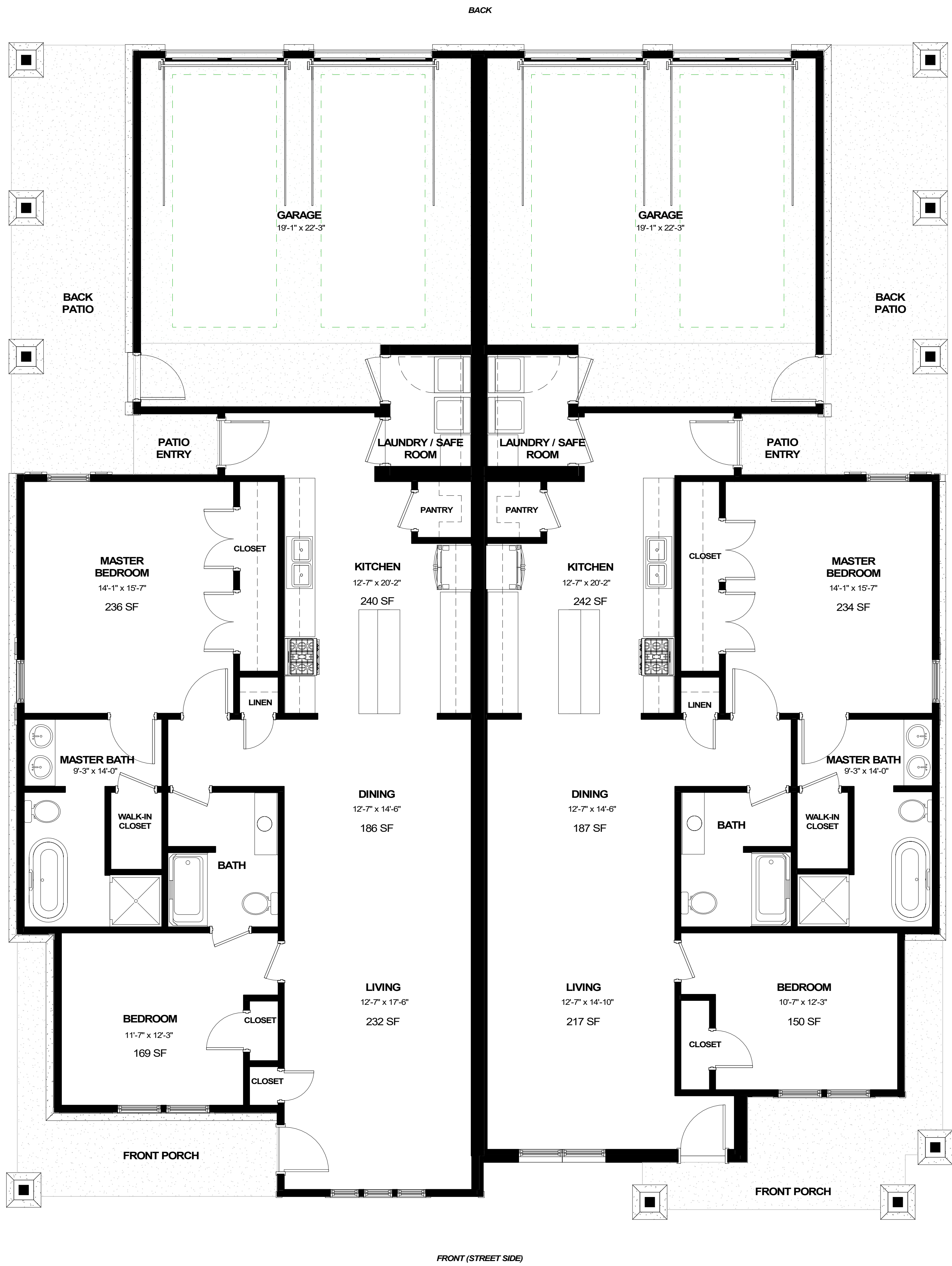
VILLA 'B' FLOOR PLAN
