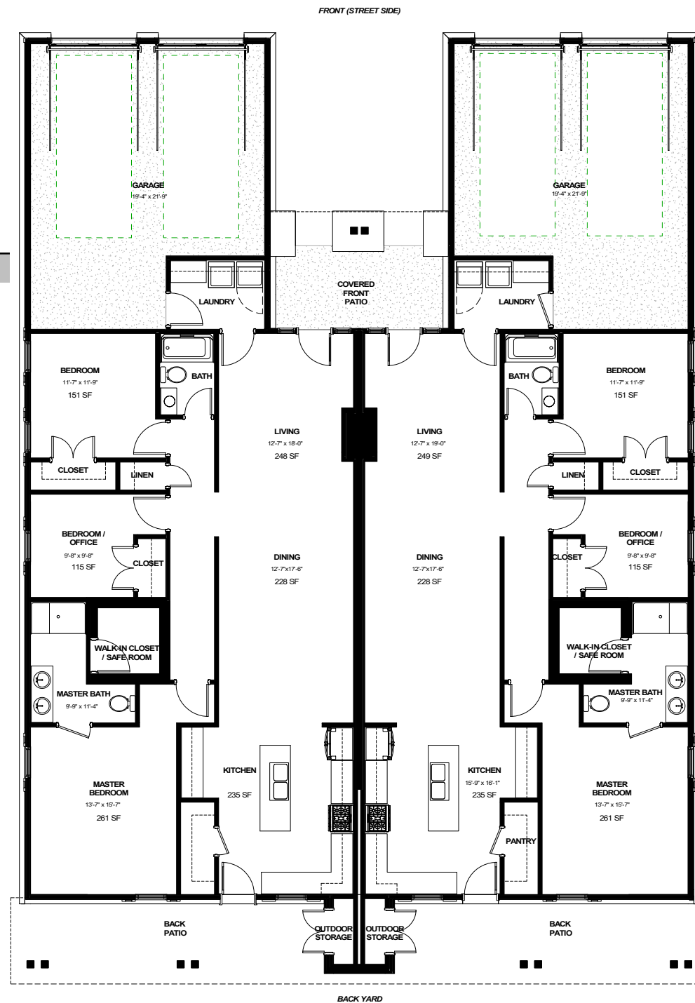
FIRST FLOOR PLAN NOT TO SCALE
