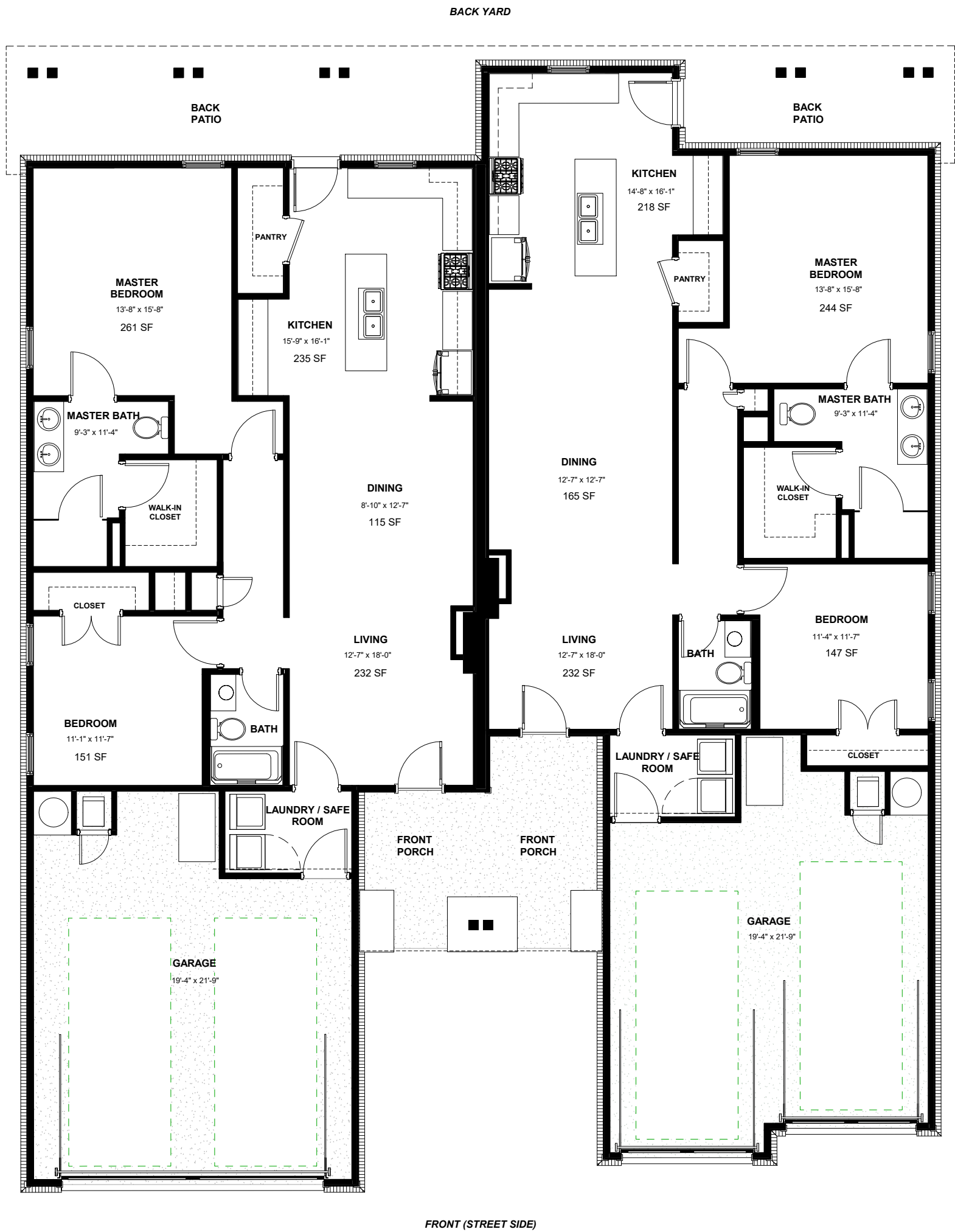
VILLA 'A' FLOOR PLAN
